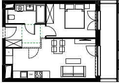
APARTMENT M2_S1 AREA: 41,93 sqm
