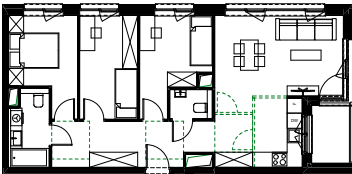
APARTMENT M4_S AREA: 71,17 sqm
